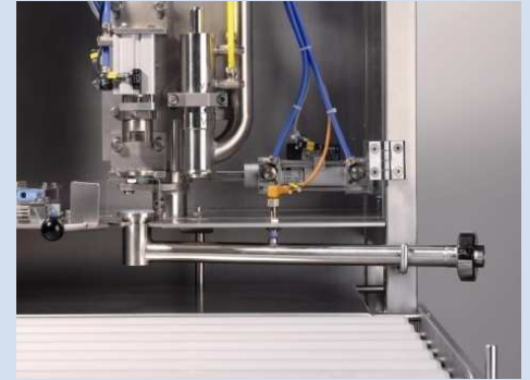
CIP – Adapter
